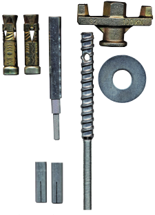
ANCHORING KIT 590 76 67-01
